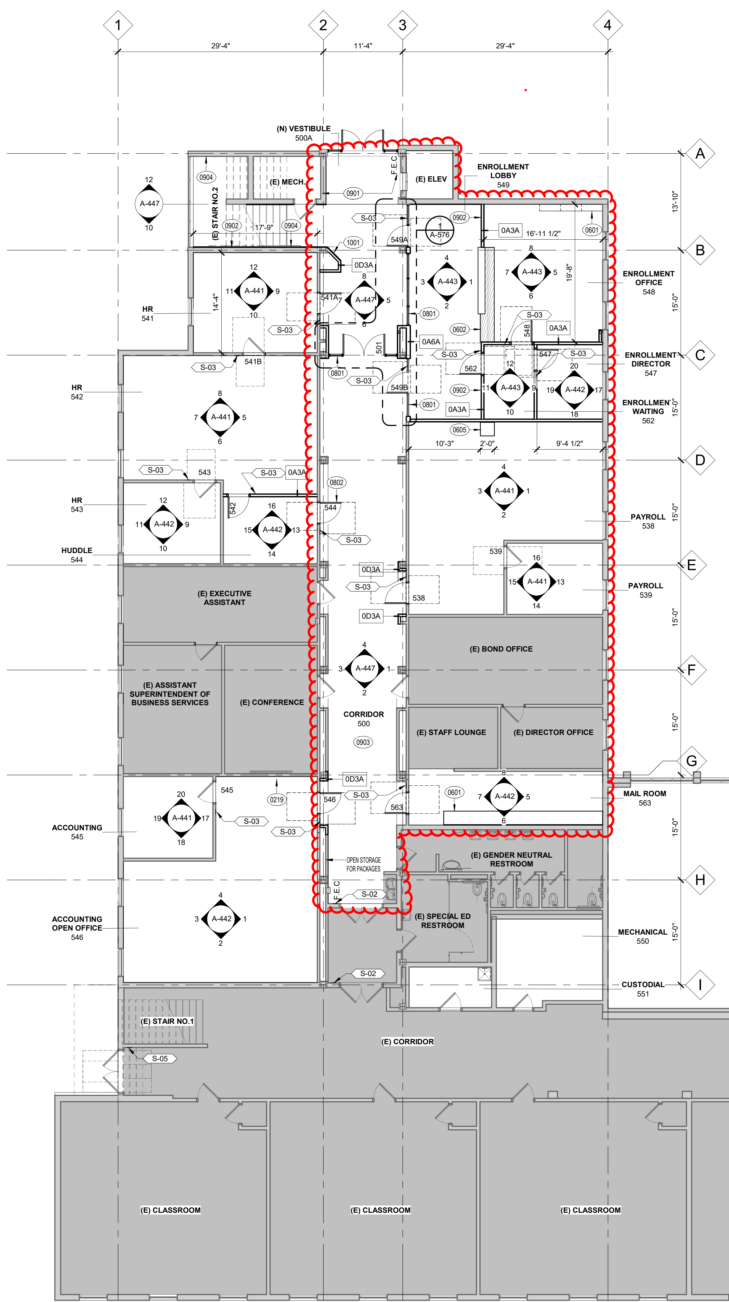
LEVEL 1 - FLOOR PLAN 1/8" = 1'-0"
