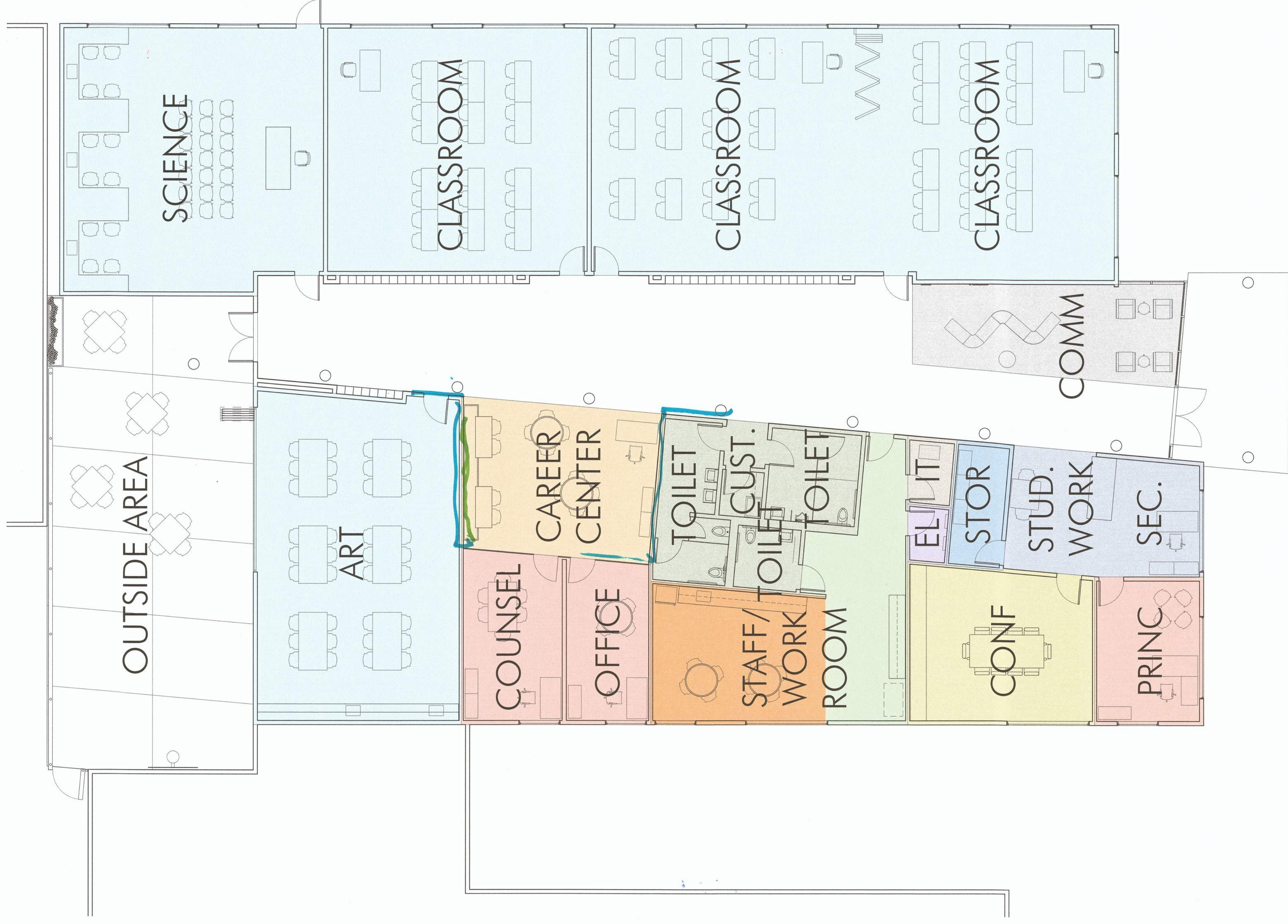
FLOOR PLAN
