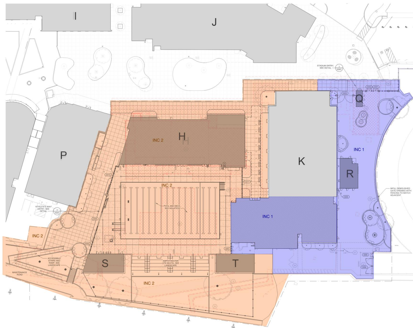
Site Plan – INC 1 & INC 2
